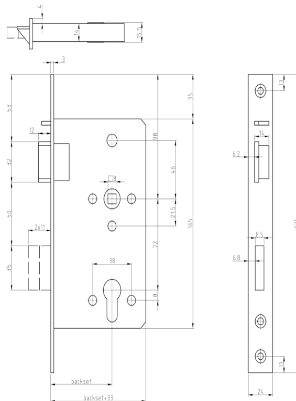
Dimensions (mm)
